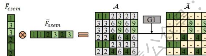
(b) Detailed illustration of "G1" within SCA in (a)
