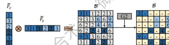
(c) Detailed illustration of "G2" within SSA in (a)
